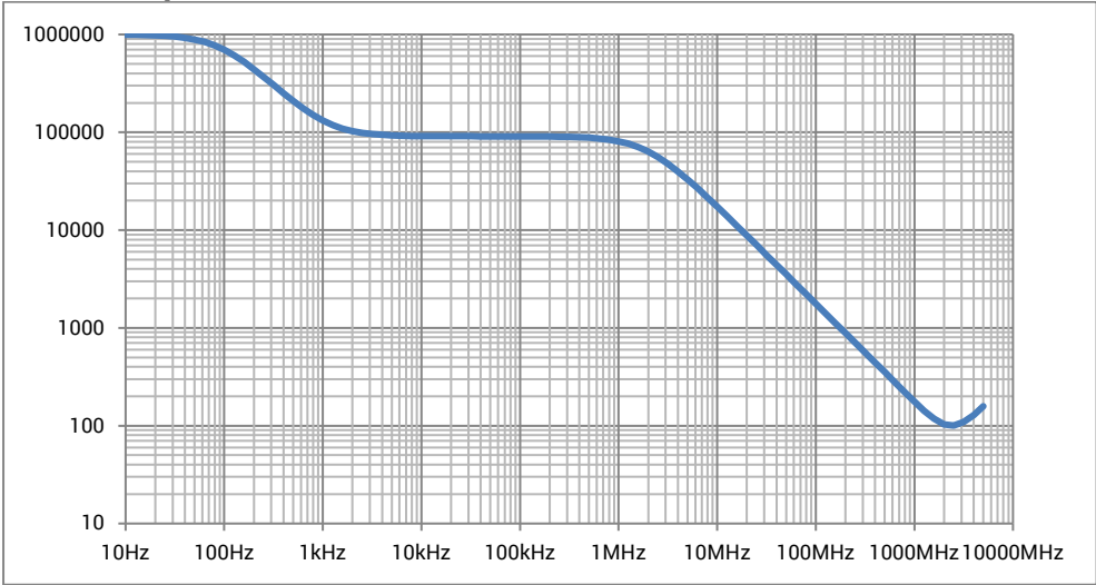
ZS1x00 Impedance Chart
